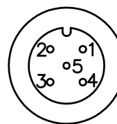
CANOPEN® ENCODERS 5-pin M12
