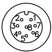
SSI ENCODERS 8-pin M12
