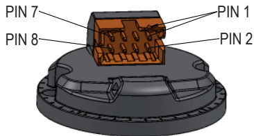
Use EPC mating cable Stock #075230
