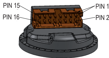
Use EPC mating cable Stock #075232
