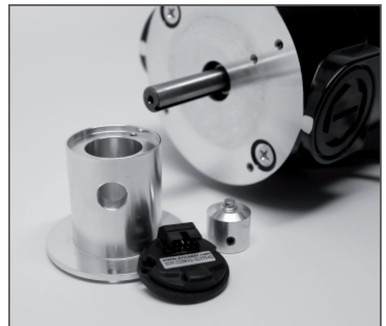
This installation is using an over-the-shaft magnet holder. This magnet holder includes a set-screw, for precise placement of the magnet on the shaft.
