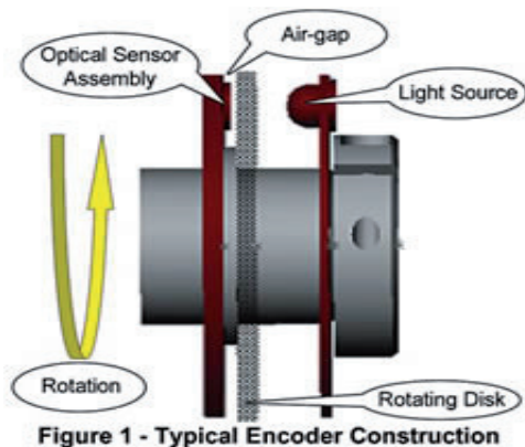
Figure 1 - Typical Encoder Construction
