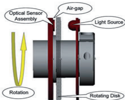
Figure 1 - Typical Encoder Construction
