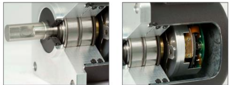
Cutaway views of Model 725i
