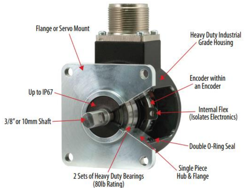
Model 725i industrial housing
